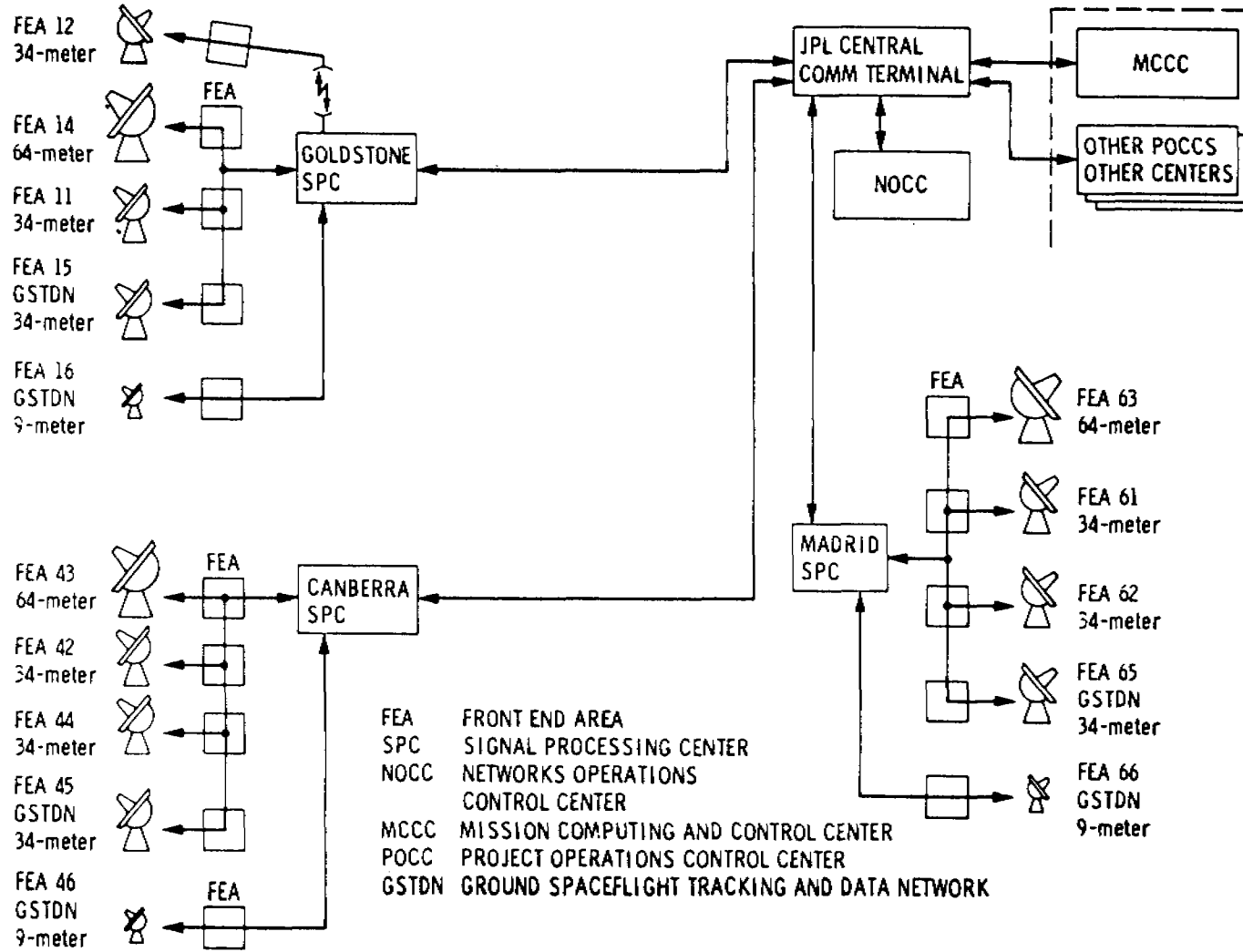
Fig. 2-Consolidated Network Configuration - 1986
